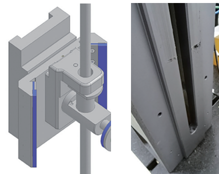
Lubricant-free guide material
